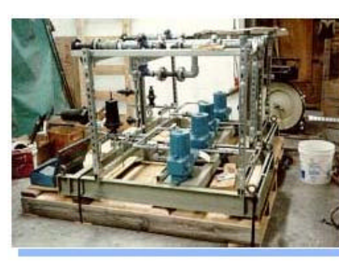
Coagulation Pumps
